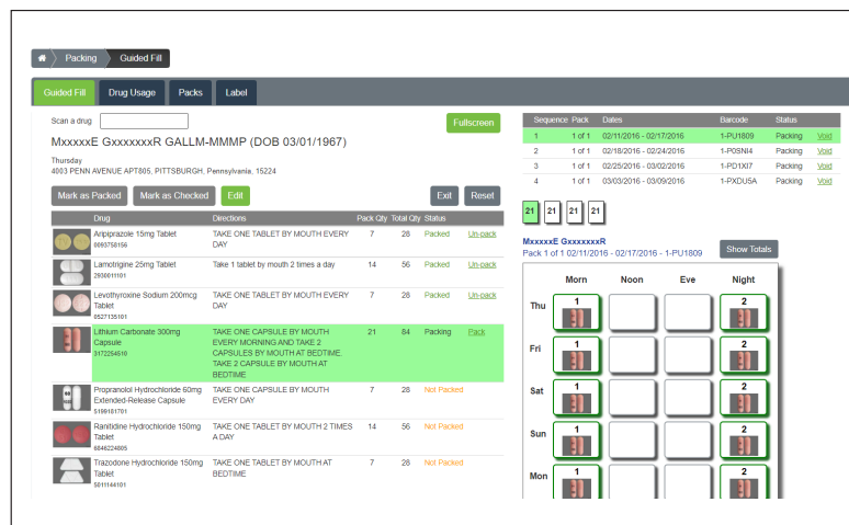
Guided Packing fill screen
